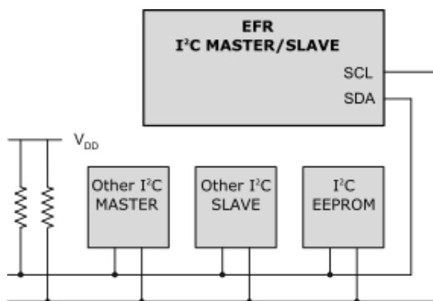
Figure 4.2. I 2 C
