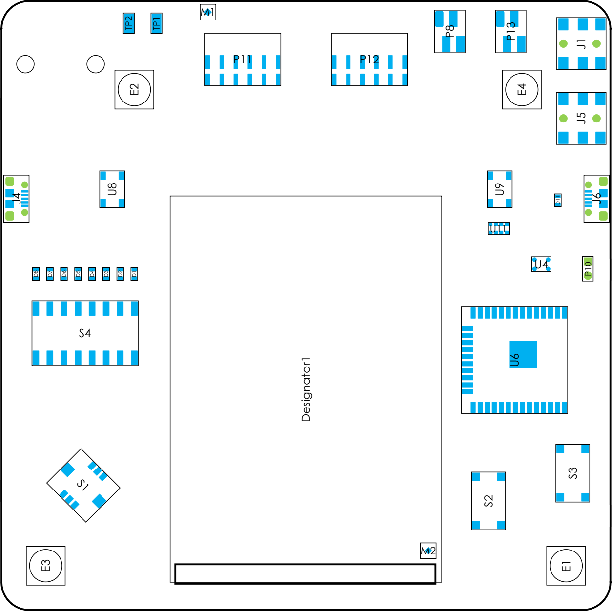
View from Top side (Scale 3:2)
